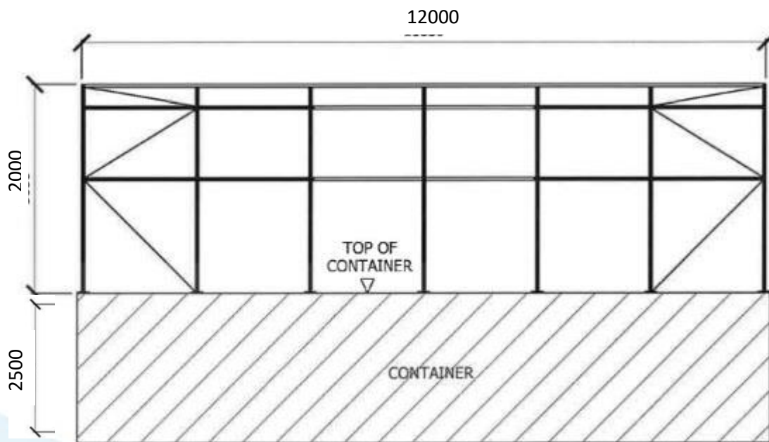
FRAMES SIDE ELEVATION
